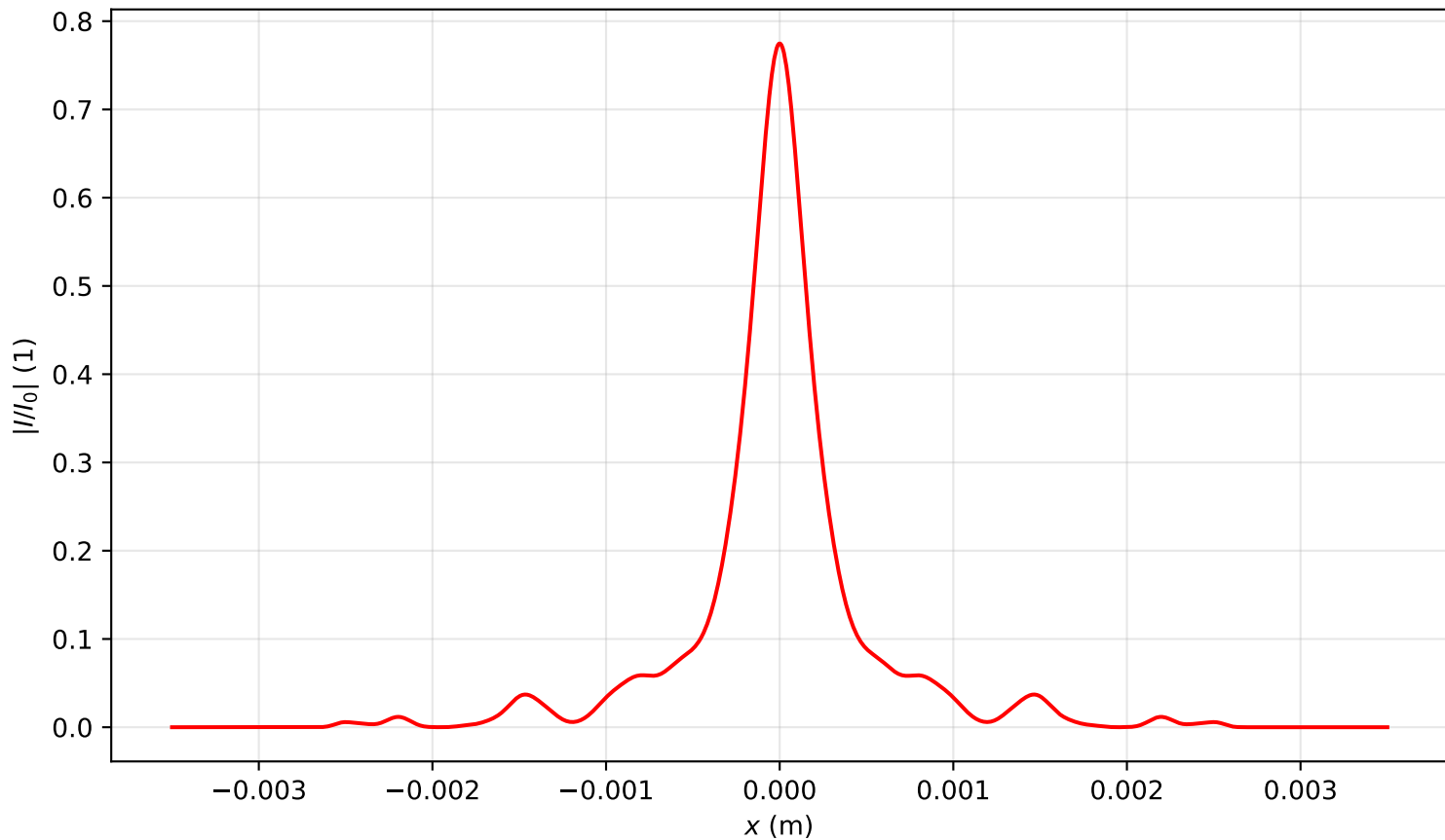
Intensity profile I(x, y = 0, z = 2.627)/I_0 , P_{in}=4.5P_{cr} , artificial time
